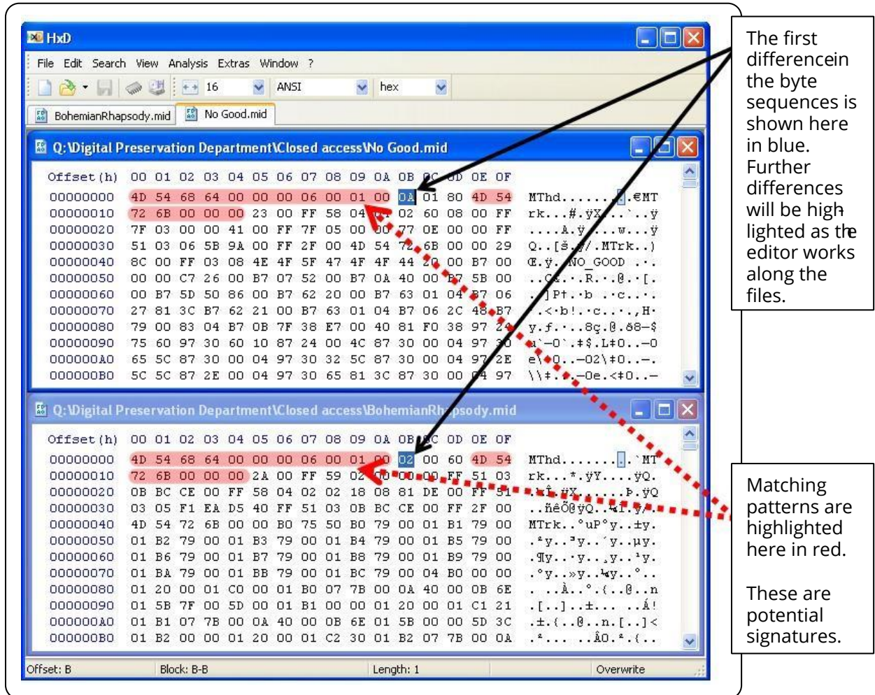
Figure 4 A hex editor being used to compare the internal structures of two MIDI files
